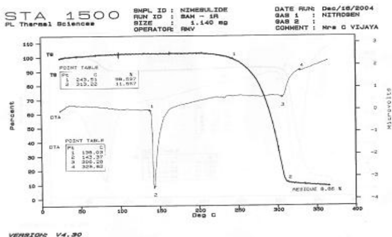
Fig. 2: Thermogram of nimesulide
