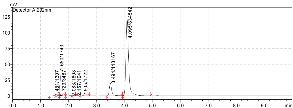
Fig. 4: Shows Acid Degraded Analytical Peak
