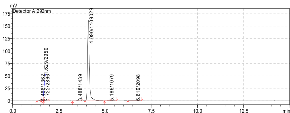
Fig. 6: Shows Oxidative Degraded Analytical Peak
