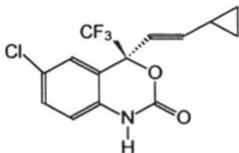
Fig. 1: Shows Structure of Efavirenz
