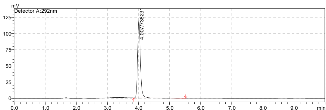
Fig. 2: Shows Chromatogram of Efavirenz 100 µg mL -1
