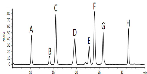
Fig. 1: HPLC chromatogram of alkaloid-rich fraction from the barks of Uncaria tomentosa L. (Rubiaceae) whereby eight alkaloids were identified, including: (A) speciophylline; (B) uncarine F; (C) mytraphylline; (D) ryncophylline; (E) isomytraphylline; (F) pteropodine; (G) isorhynchophylline; (H) isopteropodine.
