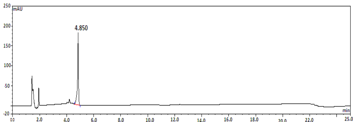
Fig. 2: HPLC chromatogram of standard negundoside
